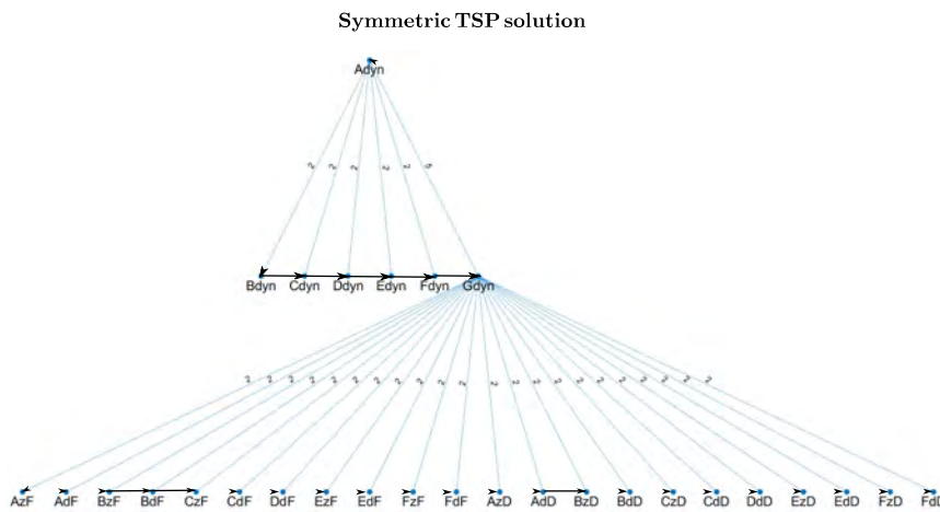
Figure 3: Solution for Symmetric TSP.
