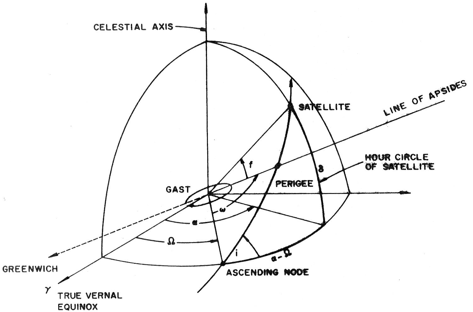
FIGURE 4-2 KEPLERIAN ORBITAL ELEMENTS
