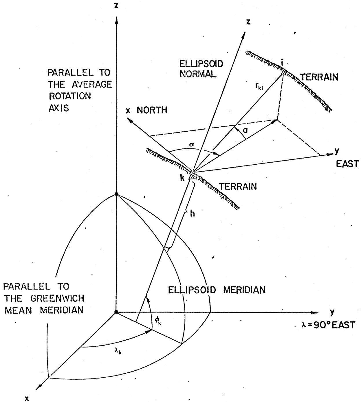
Figure 2-12 GEODETIC AND LOCAL GEODETIC COORDINATE SYSTEMS
