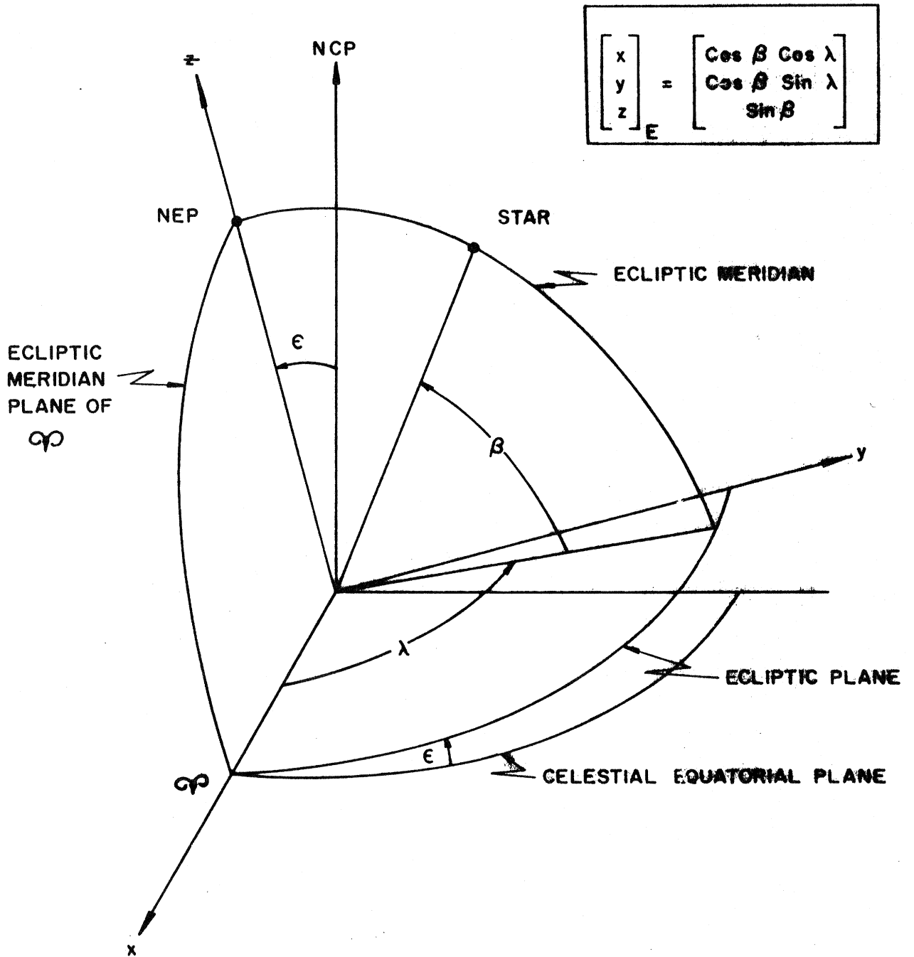
Figure 3-1. ECLIPTIC SYSTEM
