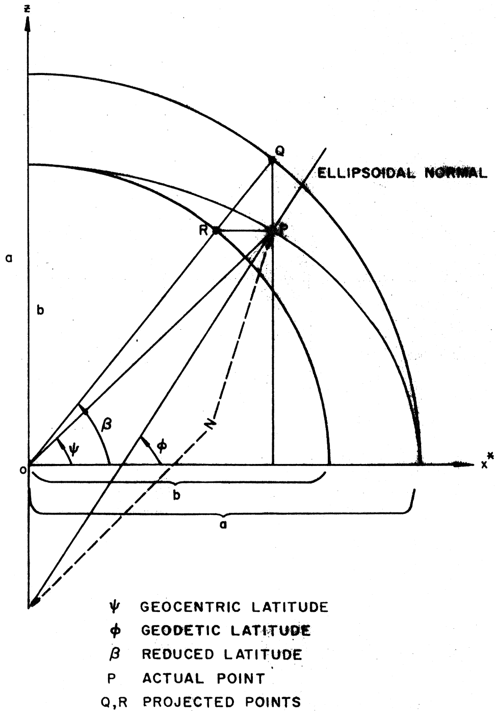
Figure 2-6. VARIOUS LATITUDES
