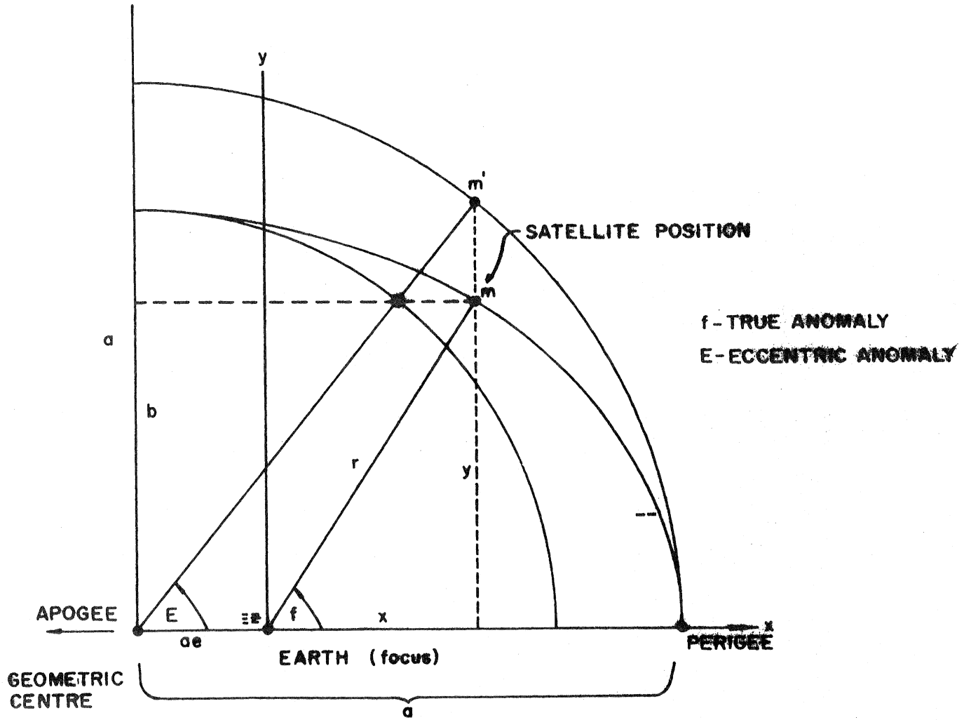
FIGURE 4-1 ORBIT ELLIPSE
