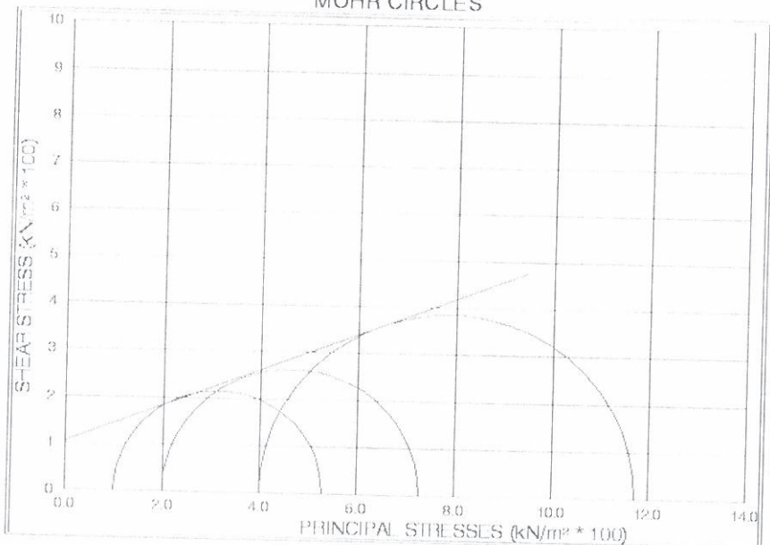
MOHR CIRCLES
